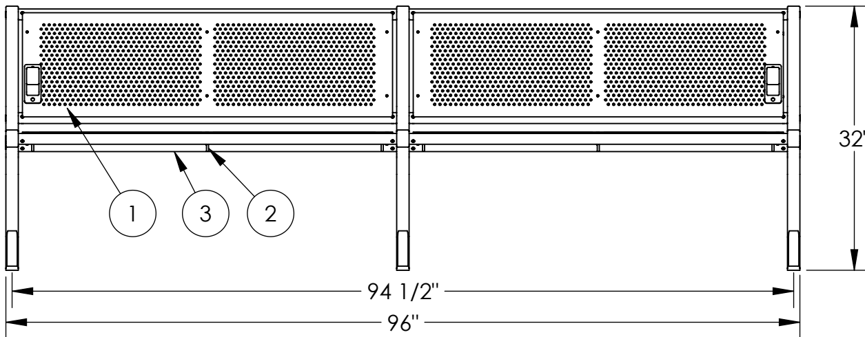
FRONT VIEW
